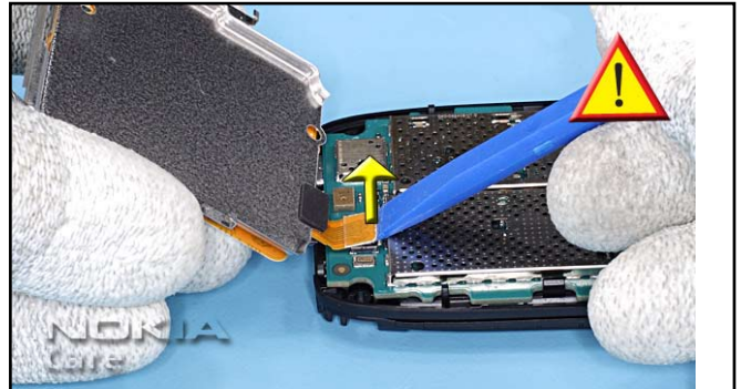
10. Gently open the UI MODULE connector, paying attention to the surrounding components.
