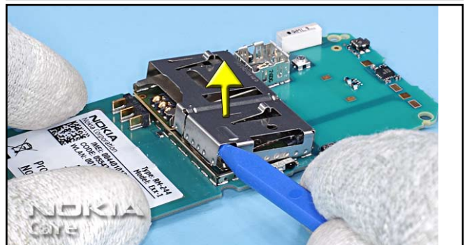
16. Remove the CARD SHIELD.
