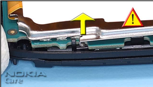
9. ...to unlock the Hook of the UI FRAME.
