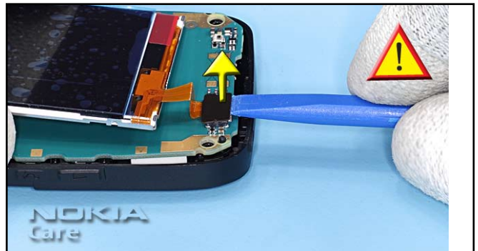
12. Gently open the DISPLAY connector, paying attention to the surrounding components.
