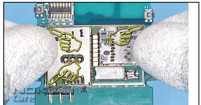
4. Align the CARD READER with the shielding lid and secure it by pressing it carefully into place.
