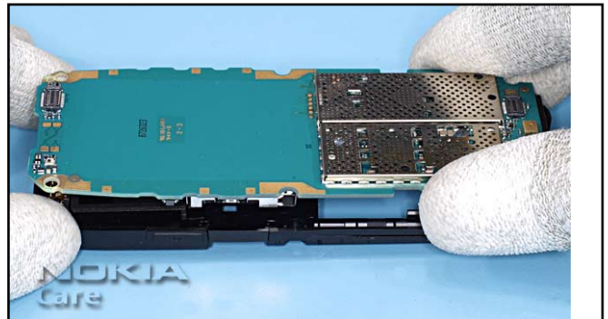
14. Remove the PWB from the B-COVER.
