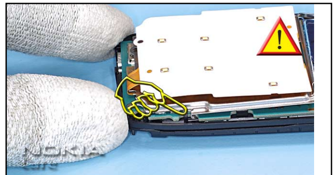
6. Attach the hook of the UI FRAME to the PWB.
